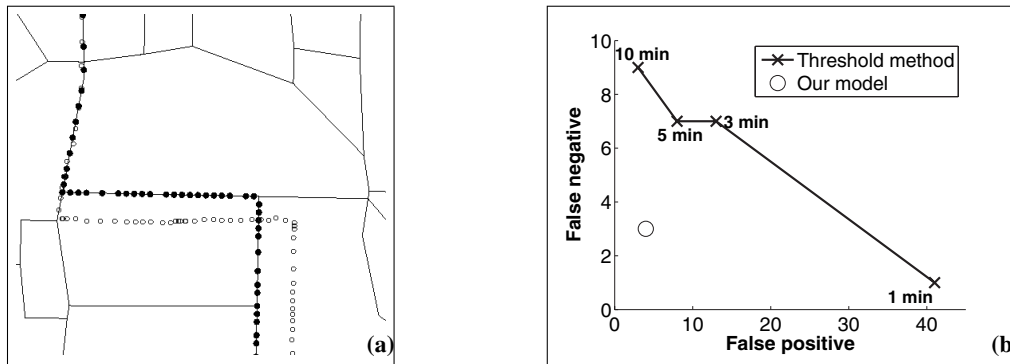
Fig. 5. (a) GPS trace (gray circles) and the associated grid cells (black circles) on the street map (lines). (b) Accuracy of extracting significant places.
