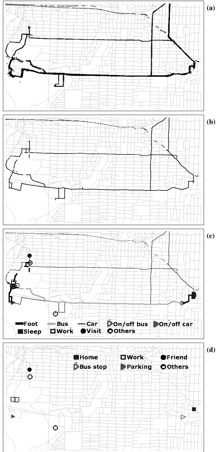
Fig. 4. Illustration of inference on part of a GPS trace, which visited this 4 km x 2 km area several times. (a) The raw GPS data has substantial variability due to sensor noise. (b) GPS trace snapped to 10 m street patches, multiple visits to the same patch are plotted on top of each other. (c) Activities estimated for each patch. (d) Places generated by clustering significant activities, followed by a determination of place types.
