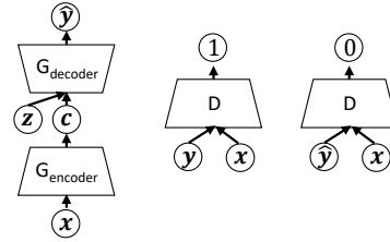
Figure 2. Architecture of SEGAN. Input of discriminator is (y, \mathbf{x}) or (\hat{y}, \mathbf{x}) ; the former should be classified as real data while the latter should be classified as fake data; but the latter should be treated as real data when updating the generator parameters, so adversarial training is performed.
