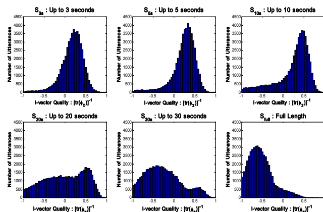
Figure 5: Histograms of the normalized i-vector quality measure for various duration conditions.
