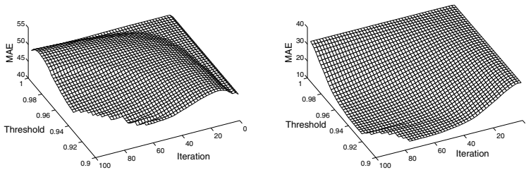
Fig. 11. Results for the datasets M1 (left) and M2 (right) for ORC
