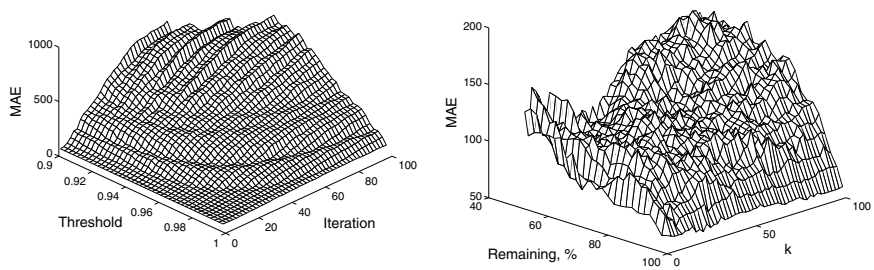
Fig. 8. Results for the dataset A1 for ORC (left) and for ODIN with K-means (right)
