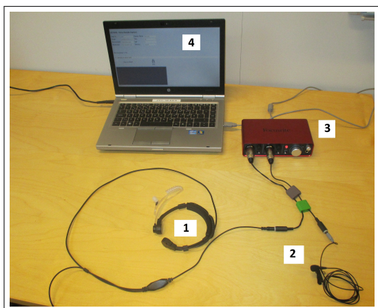
Figure 2: Data collection setup with (1) Throat microphone, (2) Close-talk or acoustic microphone, (3) USB audio interface, (4) Web-based user interface.
