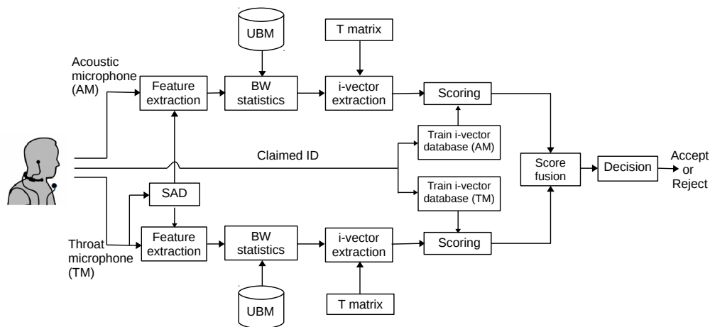
Figure 1: Block diagram of speaker recognition system with dual microphone setup.
