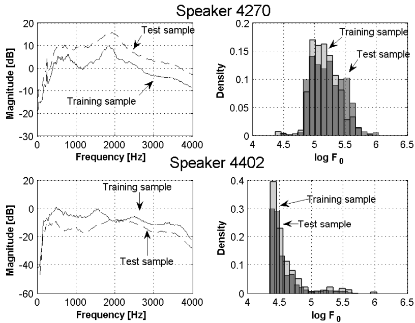
Figure 6.4: Long term average spectra (left) along with F_0 histograms (right). For two speakers recognized by F_0 but missed by MFCC
