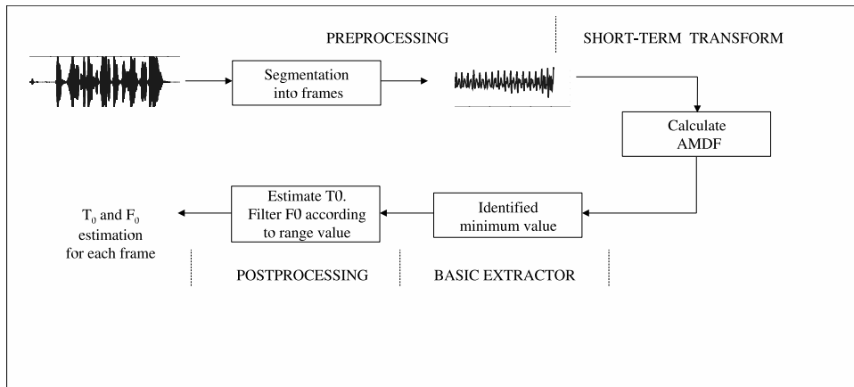
Figure 4.6: Diagram of AMDF F_0 estimation algorithm
