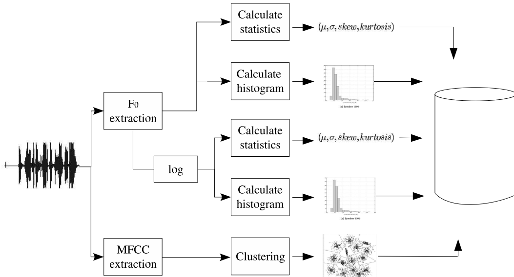
Figure 6.1: Diagram of training phase
