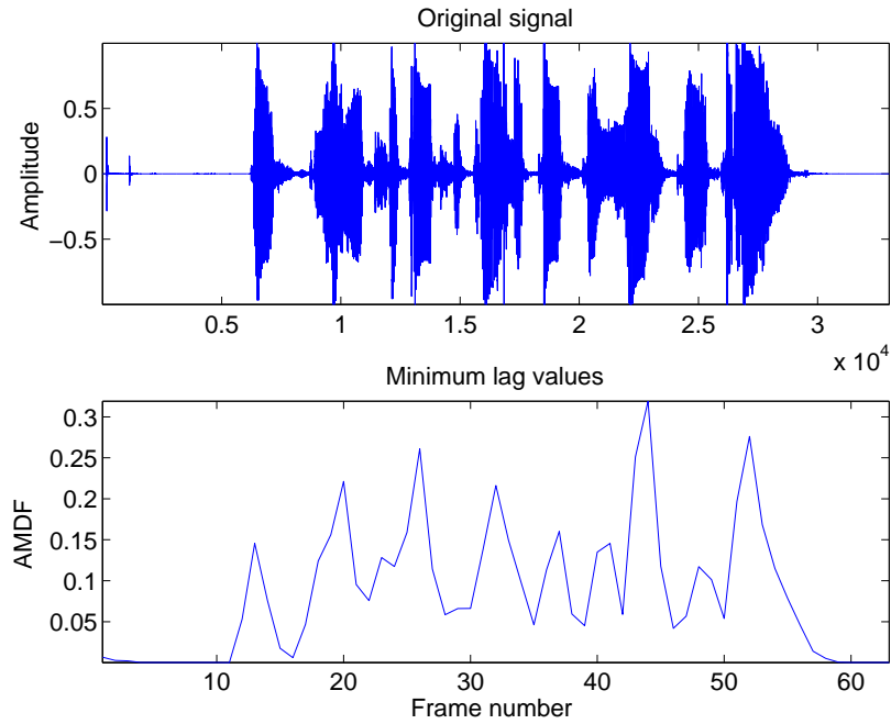
Figure 4.5: Minimum lag values for AMDF (sampling rate 16 kHz).
