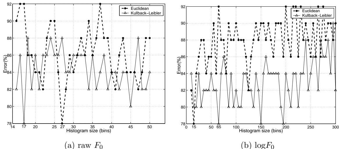
Figure 6.2: Histogram size selection
