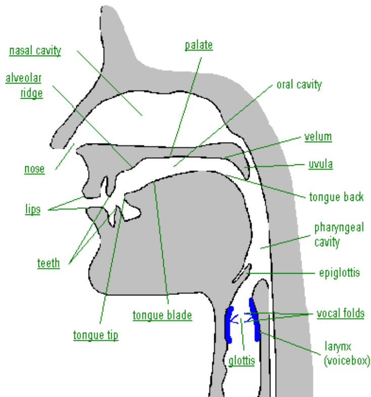
Figure 2.1: The principal organs for articulation [33].
