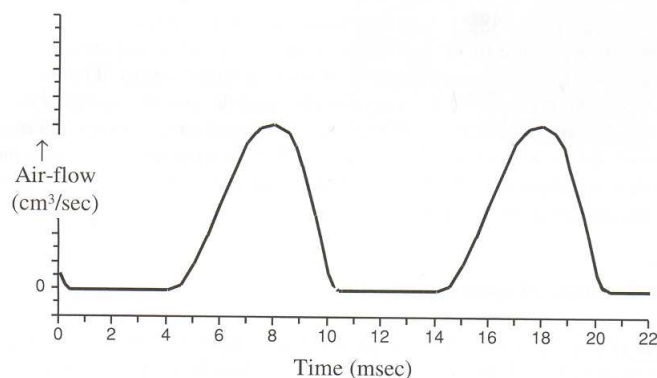
Figure 2.4: Two periods waveform of a glottal pulse [37]
