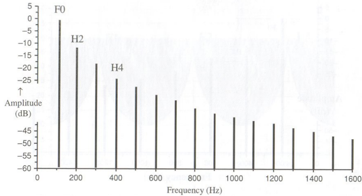
Figure 2.5: Spectrum of the glottal pulse waveform [37]
