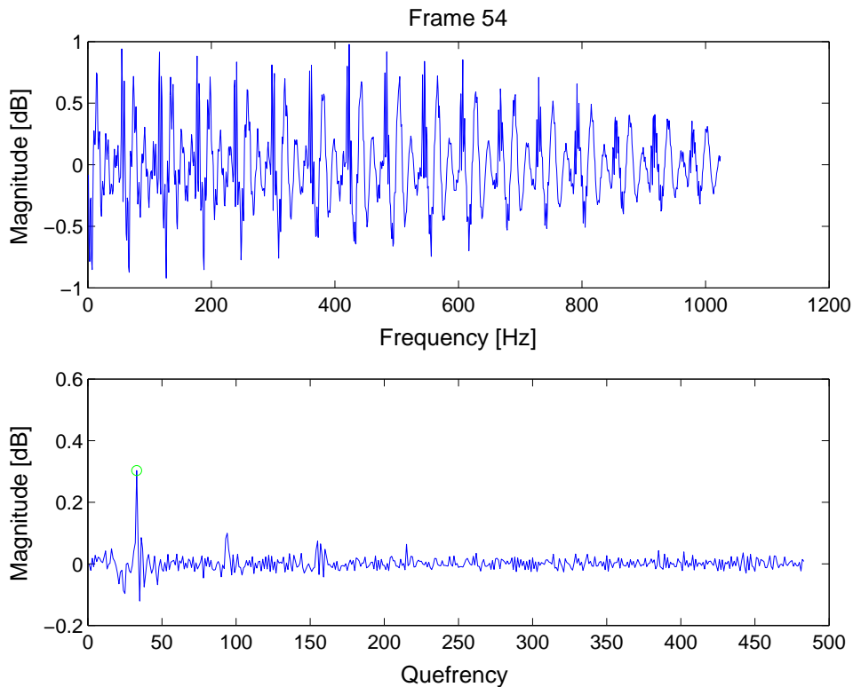
Figure 4.7: Cepstrum for voiced frame
