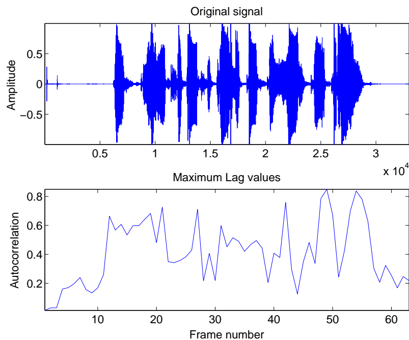
Figure 4.2: Maximum lags in autocorrelation (sampling rate 16 kHz).
