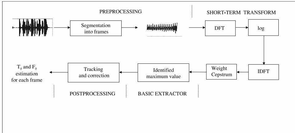
Figure 4.9: Diagram of F_0 estimation based in cepstrum analysis
