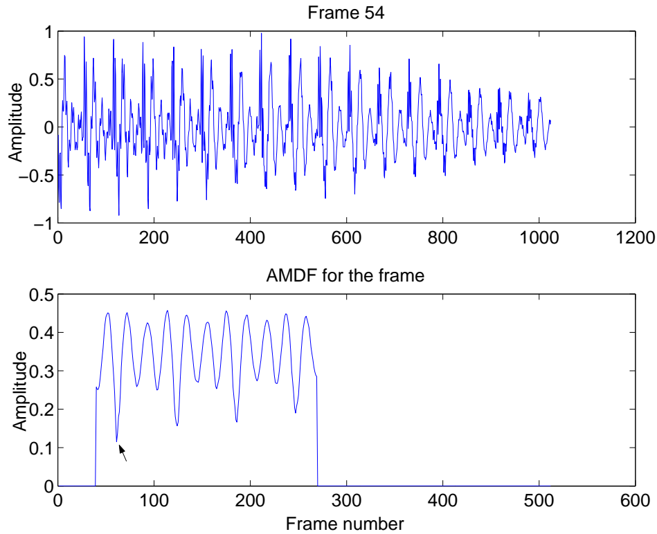
Figure 4.4: AMDF for voiced frame
