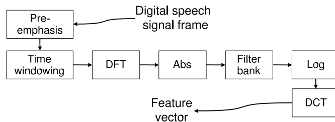
Figure 5.4: Scheme of MFCC signal processing steps [40]
