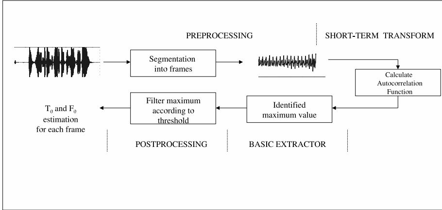
Figure 4.3: Diagram of F_0 estimation based in autocorrelation
