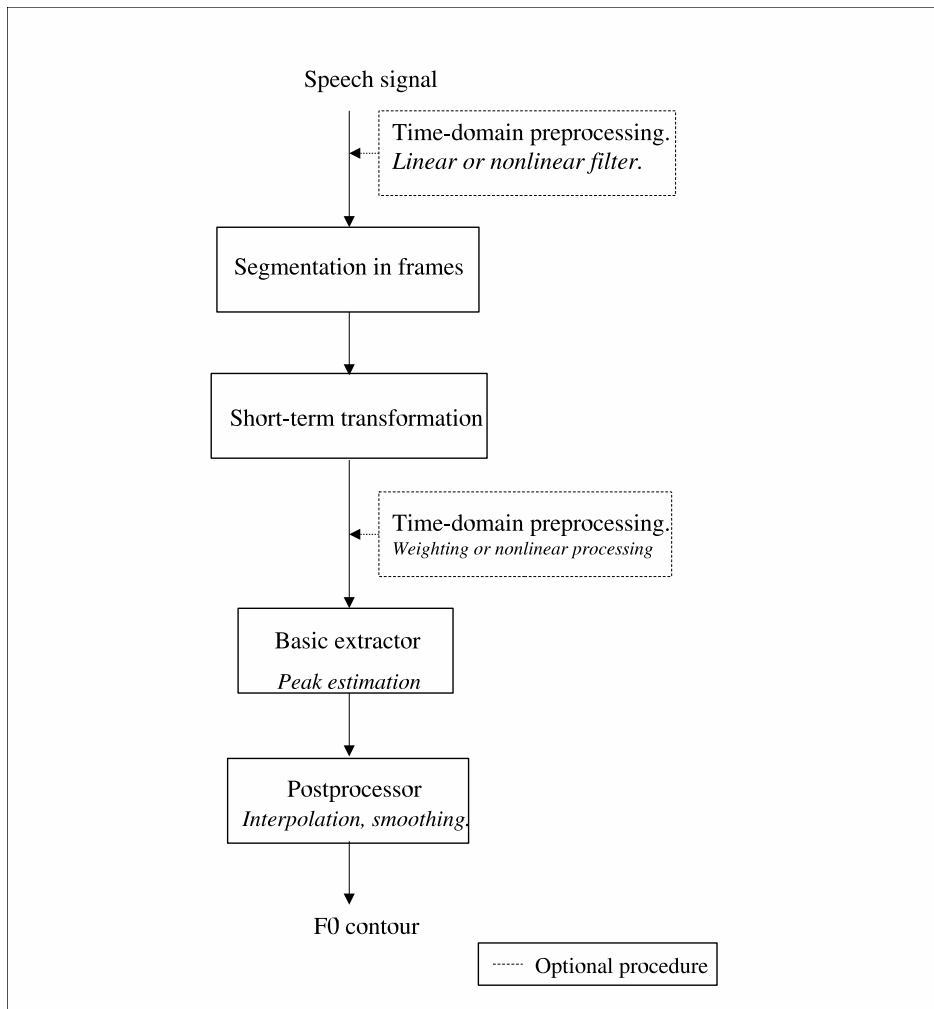
Figure 3.2: Diagram of the short-term analysis F_0 algorithm
