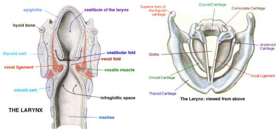
Figure 2.2: Diagrams with views of the larynx [14].
