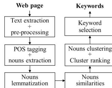
Figure 2. Keyword extraction algorithm.
