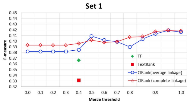
Figure 4. Average F-measure results with set 1.
