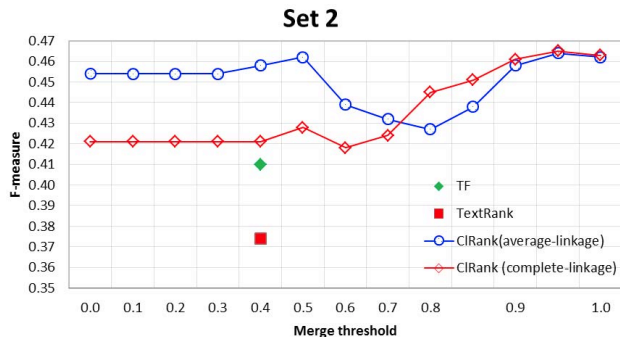
Figure 5. Average F-measure results with set 2.
