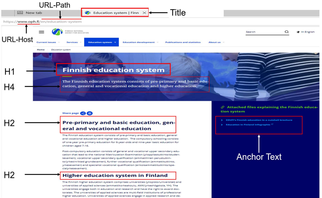
Fig. 1. Title, URL, and the structure of an example web page.
