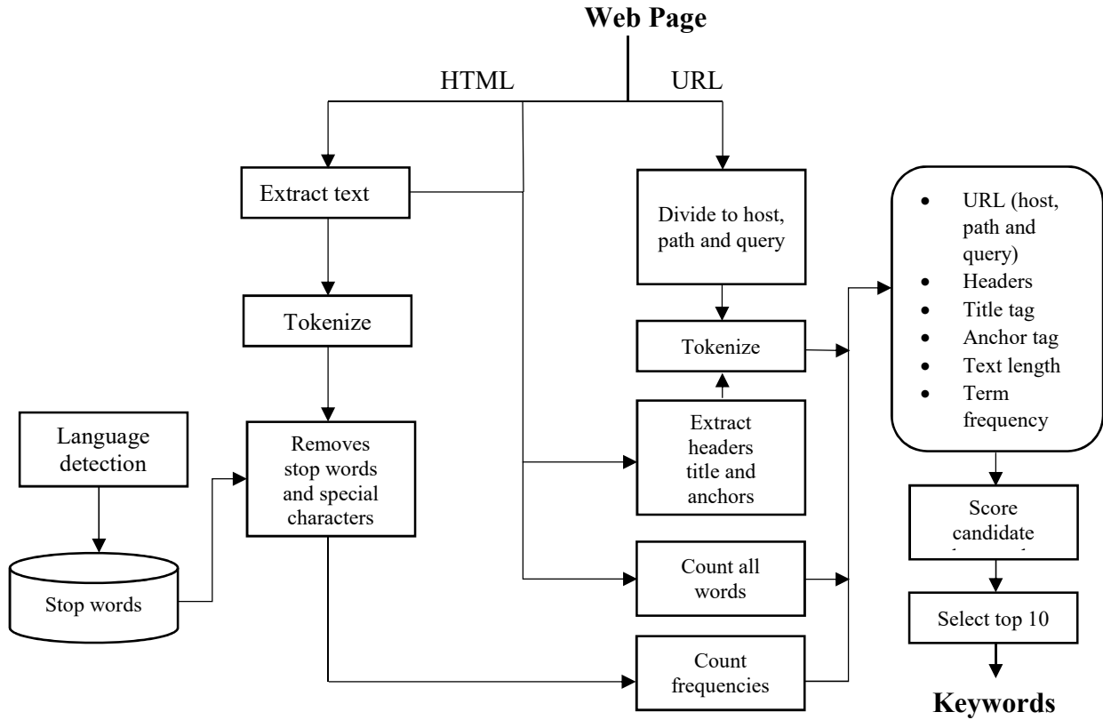
Fig. 2. Workflow of the proposed D-rank
