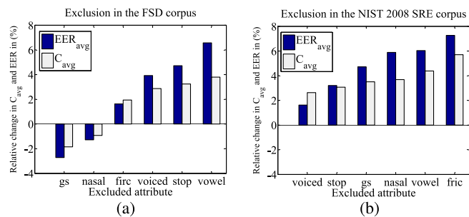
Fig. 9. Exclusion experiment: relative change in the error rates as one attribute is left out. Positive relative change indicates increment in the error rates. (a) FSD task. (b) NIST 2008 task.
