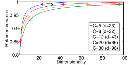
Fig. 3. Remaining variance after PCA. Comparing stacked context sizes ( C ) 5, 8, 12, 20 and 30 frames for manner attributes. d varies from \sim 20 to \sim 100 , with larger dimensionality assigned to longer context sizes.
