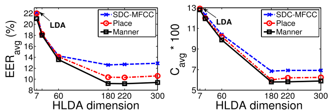
Fig. 5. Recognition error rates as a function of HLDA dimension on the FSD corpus. I-vectors are of dimensionality 1000. For lower HLDA dimensions, i.e., 7, 20 and 60, the systems attain lower recognition accuracies.
