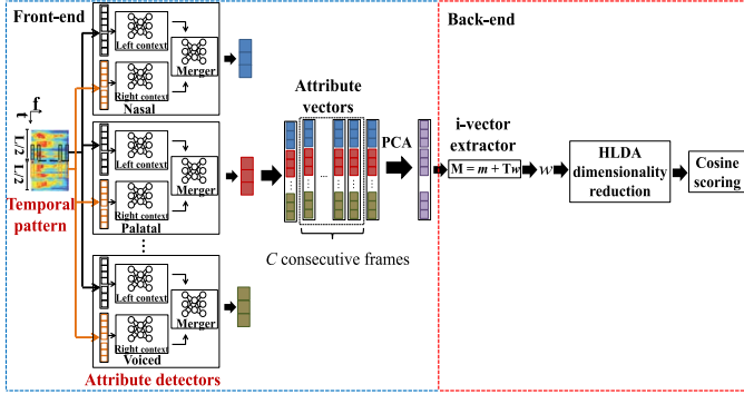
Fig. 2. Block diagram of the proposed system. In the attribute detectors [29], [30], [27], spectral features are fed into left-context and right-context artificial neural networks. A merger then combines the outputs generated by those two neural networks and produce the final attribute posterior probabilities. Principal component analysis (PCA) is then applied on C consecutive frames of these posterior probabilities to create long-term contextual features. We use i-vector approach [33] with cosine scoring [33] to classify target accents.
