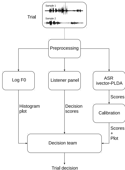
Figure 1: Fusion strategy components.
