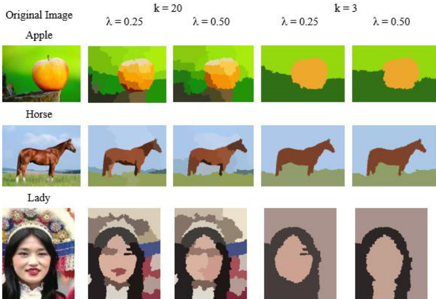
Figure 2. Examples of the effect of \lambda on the segmentation result.
