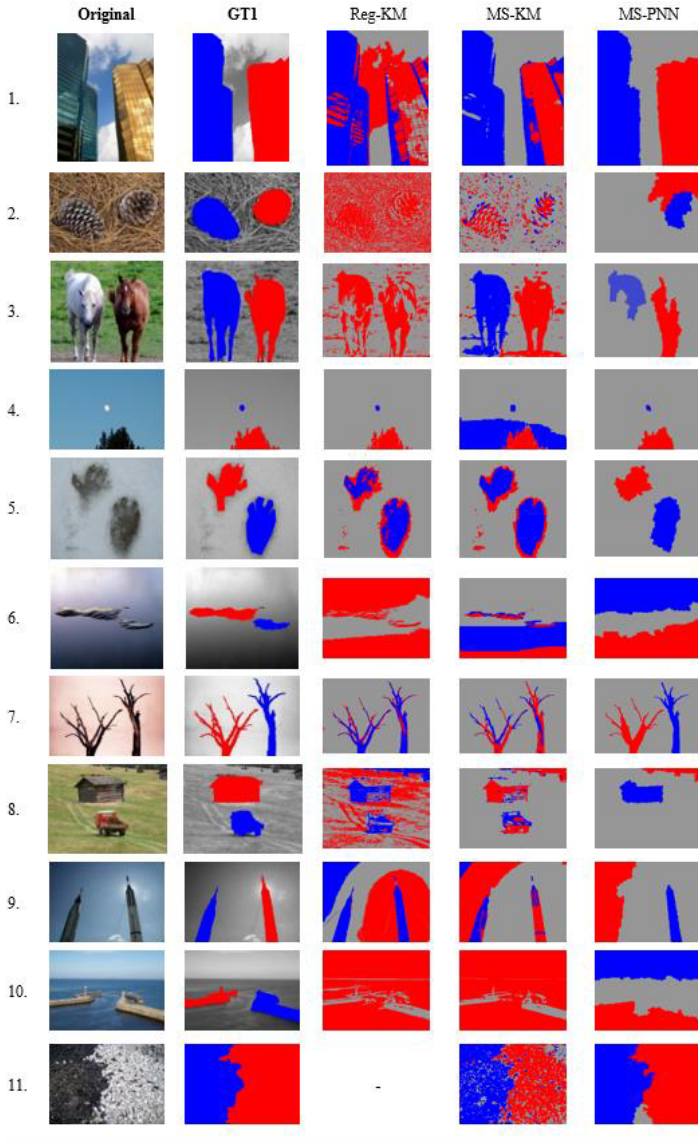
Figure 1. Visual comparison of the segmentation results using three methods.
