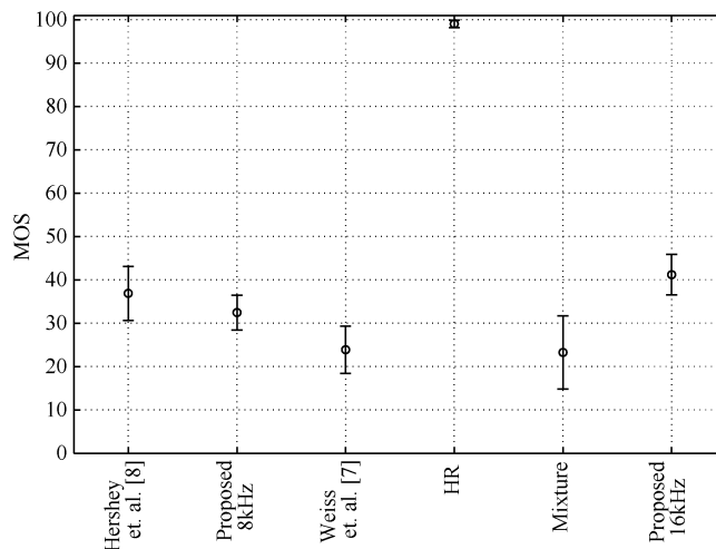
Fig. 9. Results of the MUSHRA listening test for different separation methods averaged over all excerpts and listeners. Error bars indicate 95% confidence intervals.
