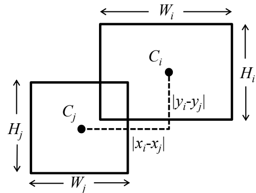
Figure 5. Overlap of the bounds of two icons
