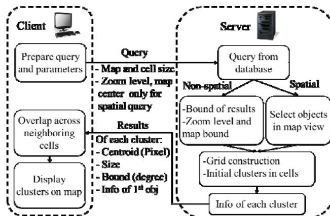
Figure 11. The proposed server-side clustering approach
