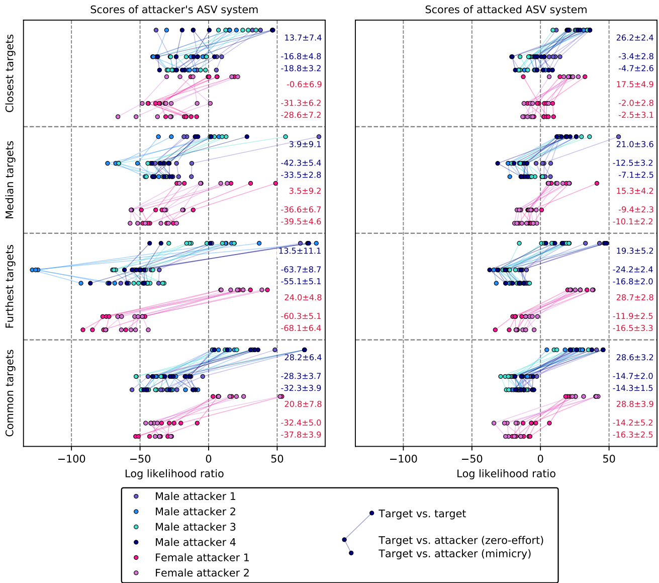
Figure 6: The scores of the ASV systems for the trials used in the listening test. The scores in each score triplet (described in the legend) are from the trials that have the same target speaker enrollment utterance and the speech content is the same in all the three test segments. Scores for male and female attackers are shown in separate groups. The right side of each graph displays the mean values of the score groups together with standard error of the mean multiplied by 1.96.
