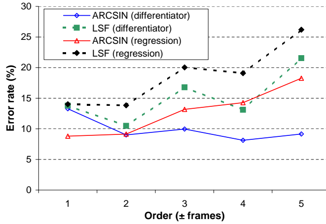
Figure 7.20: Comparison of the differentiator and regression method on the TIMIT corpus.
