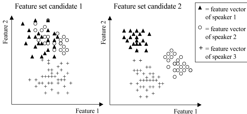
Figure 2.2: Examples of two-dimensional feature sets with poor and good discrimination.
