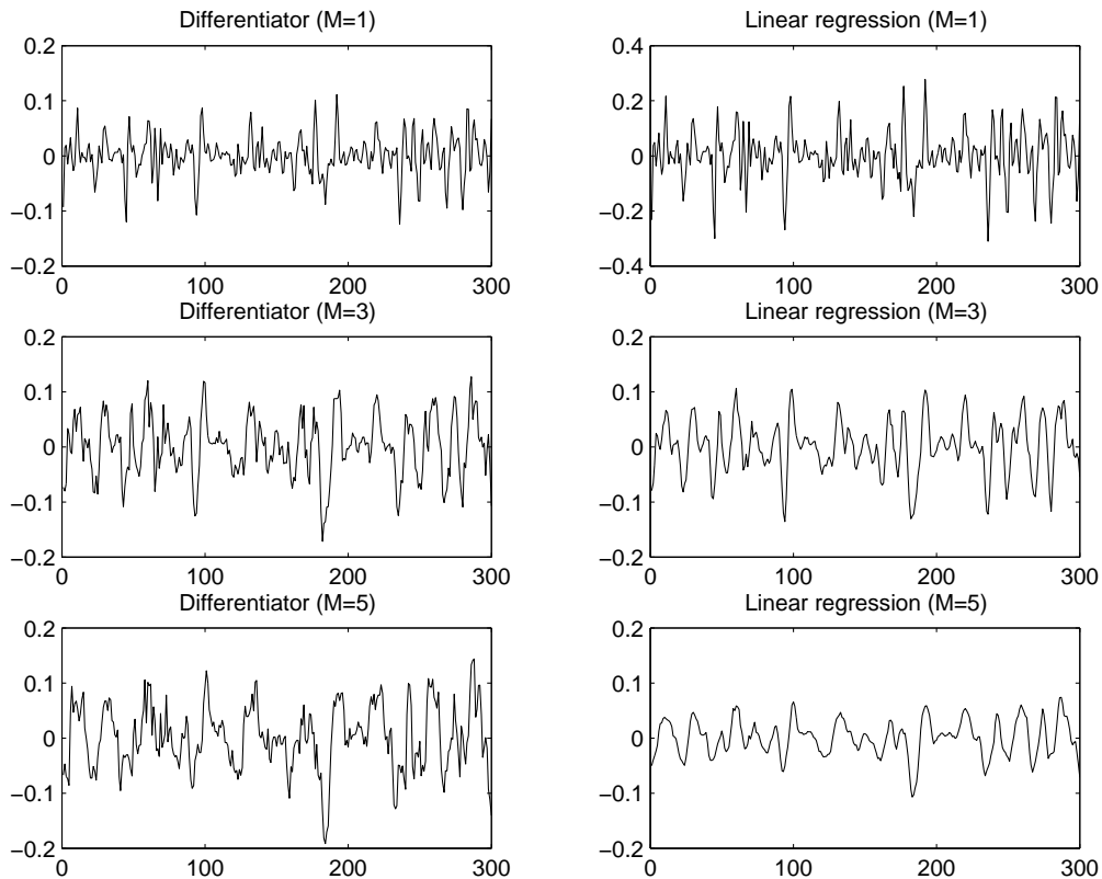
Figure 5.11: Comparison of derivative estimation using differentiator and linear regression with different orders.
