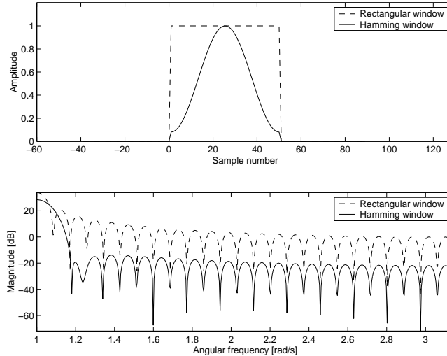
Figure 4.3: Waveforms and magnitude responses of rectangular and Hamming windows estimated by the DFT.
