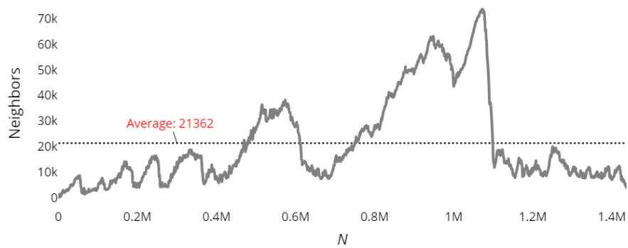
Figure 3. The development of neighborhood size during the initialization process ( n = 1.4\text{M} ).
